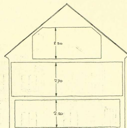
Skärning.
